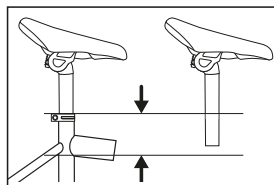
Fig. 3: Saddle height / minimum insertion depth
